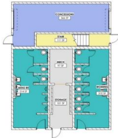
ATHLETICS PRESSBOX - FIRST FLOOR PLAN 1/8" = 1'-0" (A1.19)
