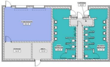
ATHLETICS CONCESSIONS 1/8" = 1'-0" (A1.19)
