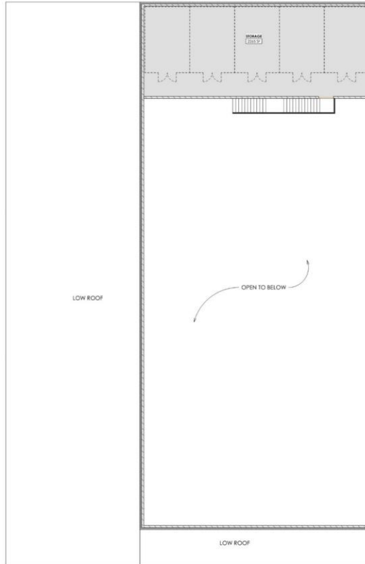
ATHLETICS FIELD HOUSE 2ND FLOOR PLAN 3/32" = 1'-0" (A1.19)
